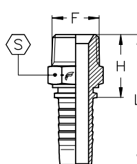
SK20 Two-Piece insert
