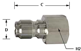
Nipple - Female
