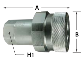
COUPLER - FEMALE
