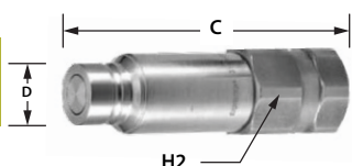
NIPPLE - FEMALE
