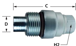
NIPPLE - FEMALE
