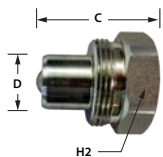
NIPPLE - BALL
