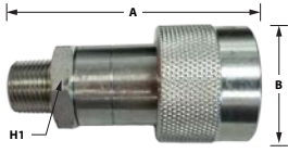
COUPLER - POPPET
